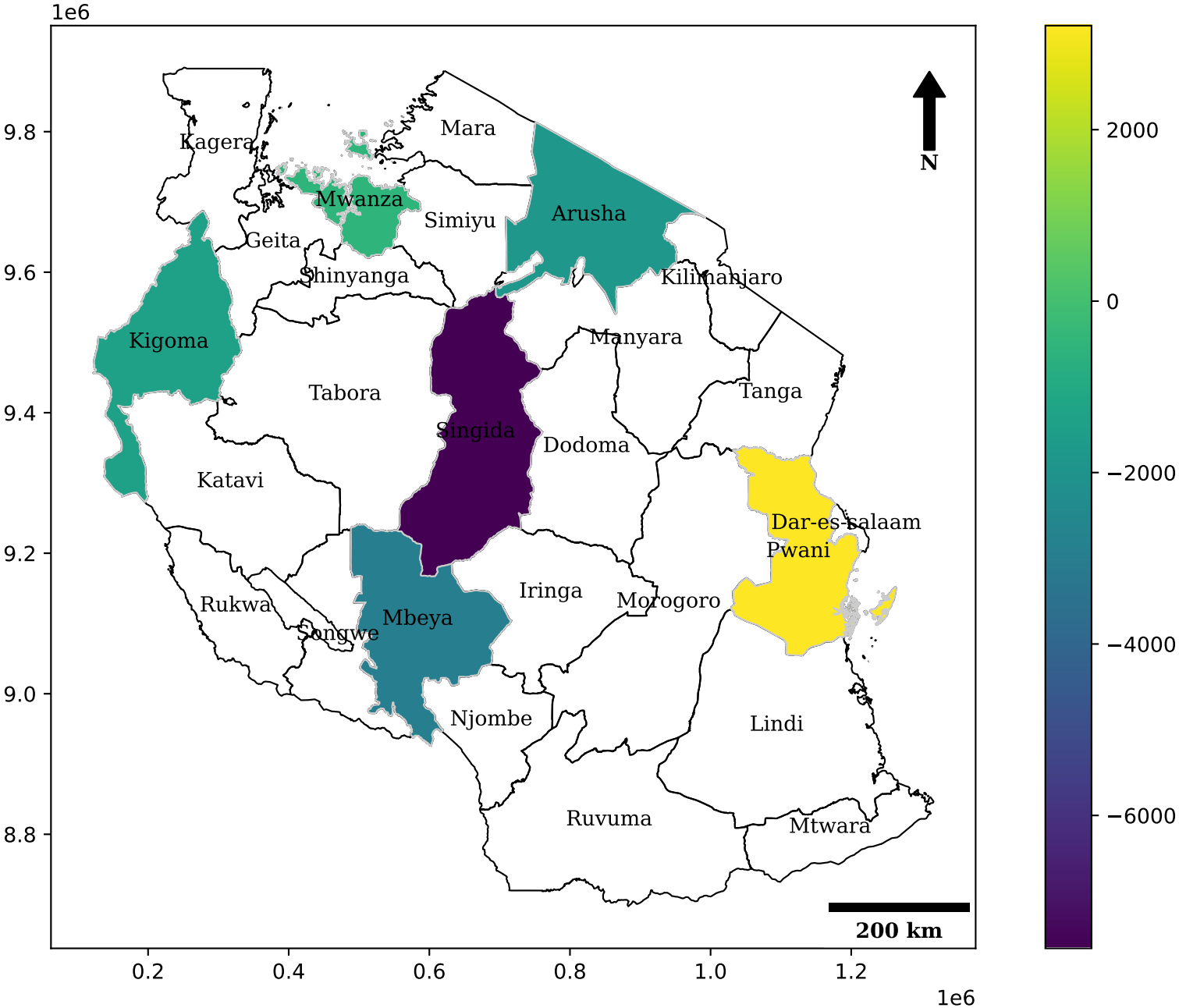
Spatial Distribution of Range Land Change (km 2 ) in Tanzania
