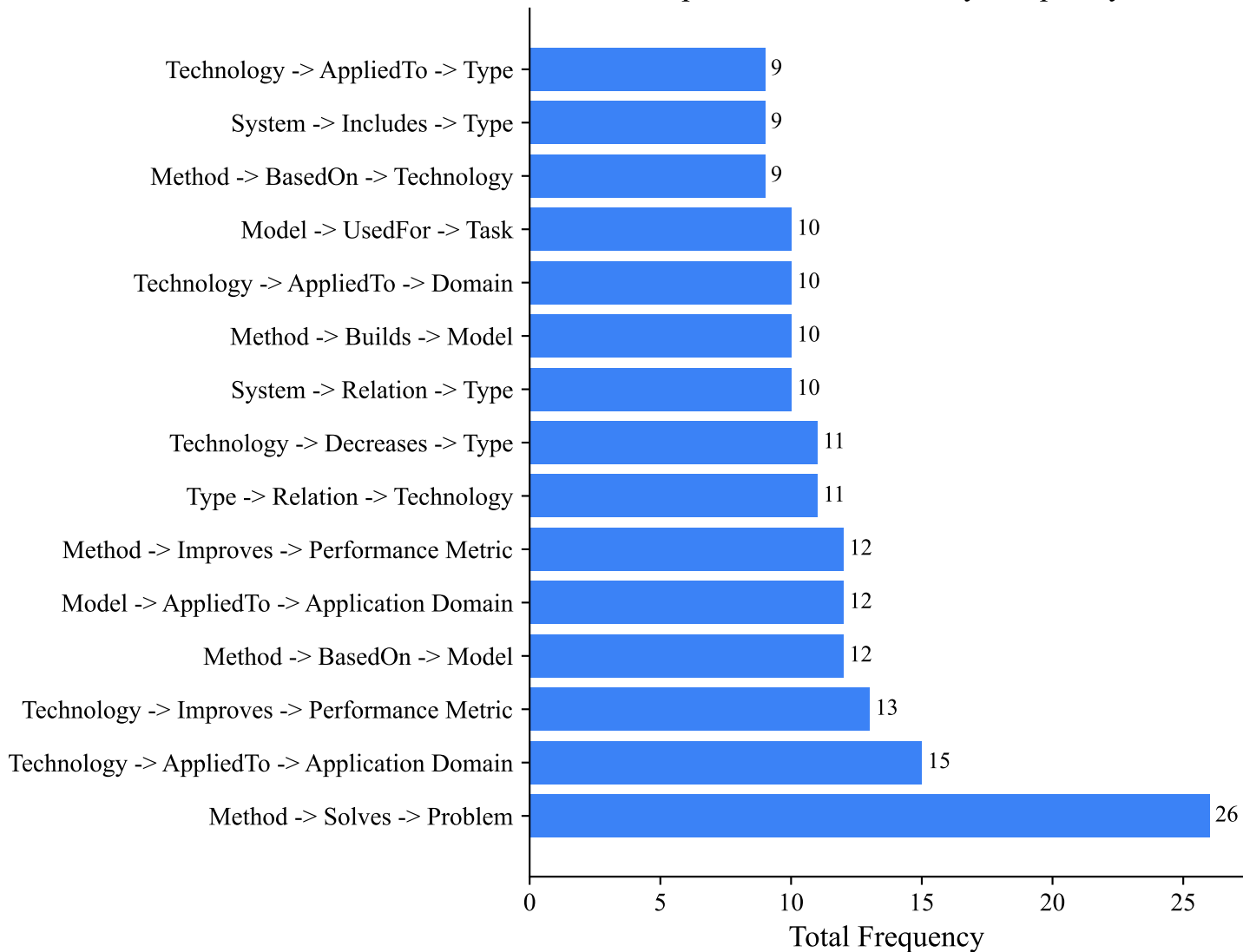
Top Semantic Patterns by Frequency
