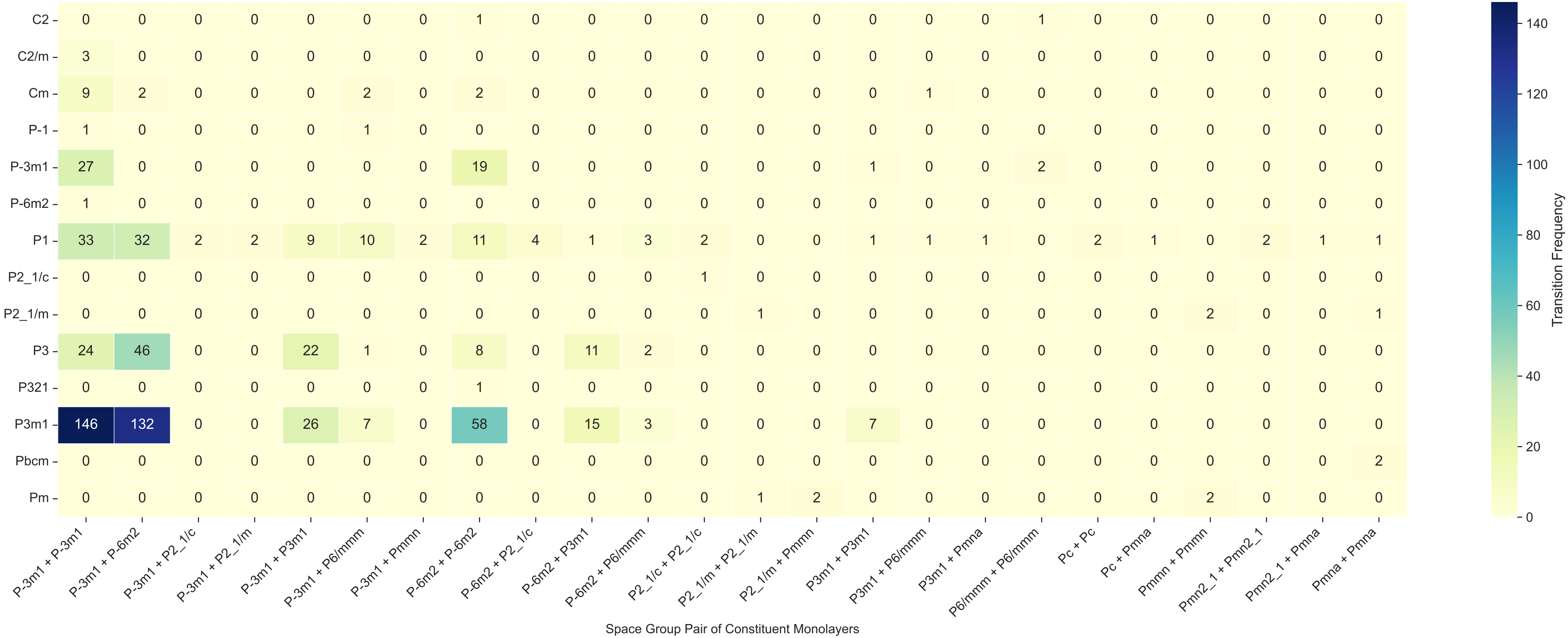
Heat Map of Symmetry Transitions: Monolayers to Bilayers
