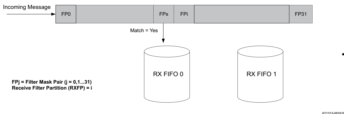
Figure 2-1: Normal Operation (RX FIFO-0)
