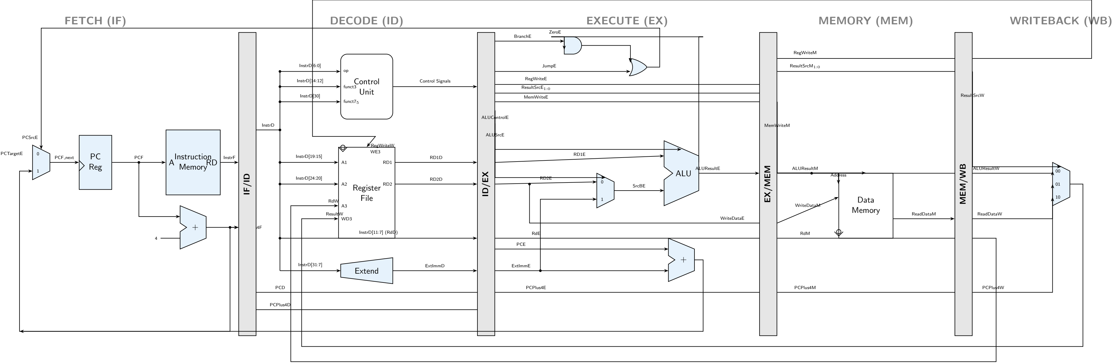
Diagrama de Datapath Pipelined Base (sin la Hazard Unit)
