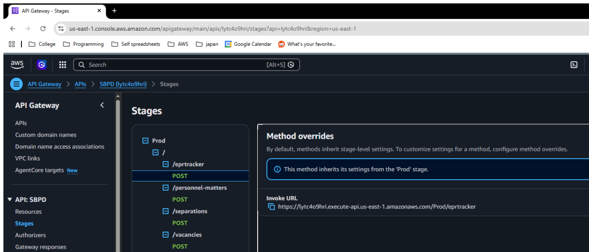
Figure 43: AWS API Gateway endpoints
