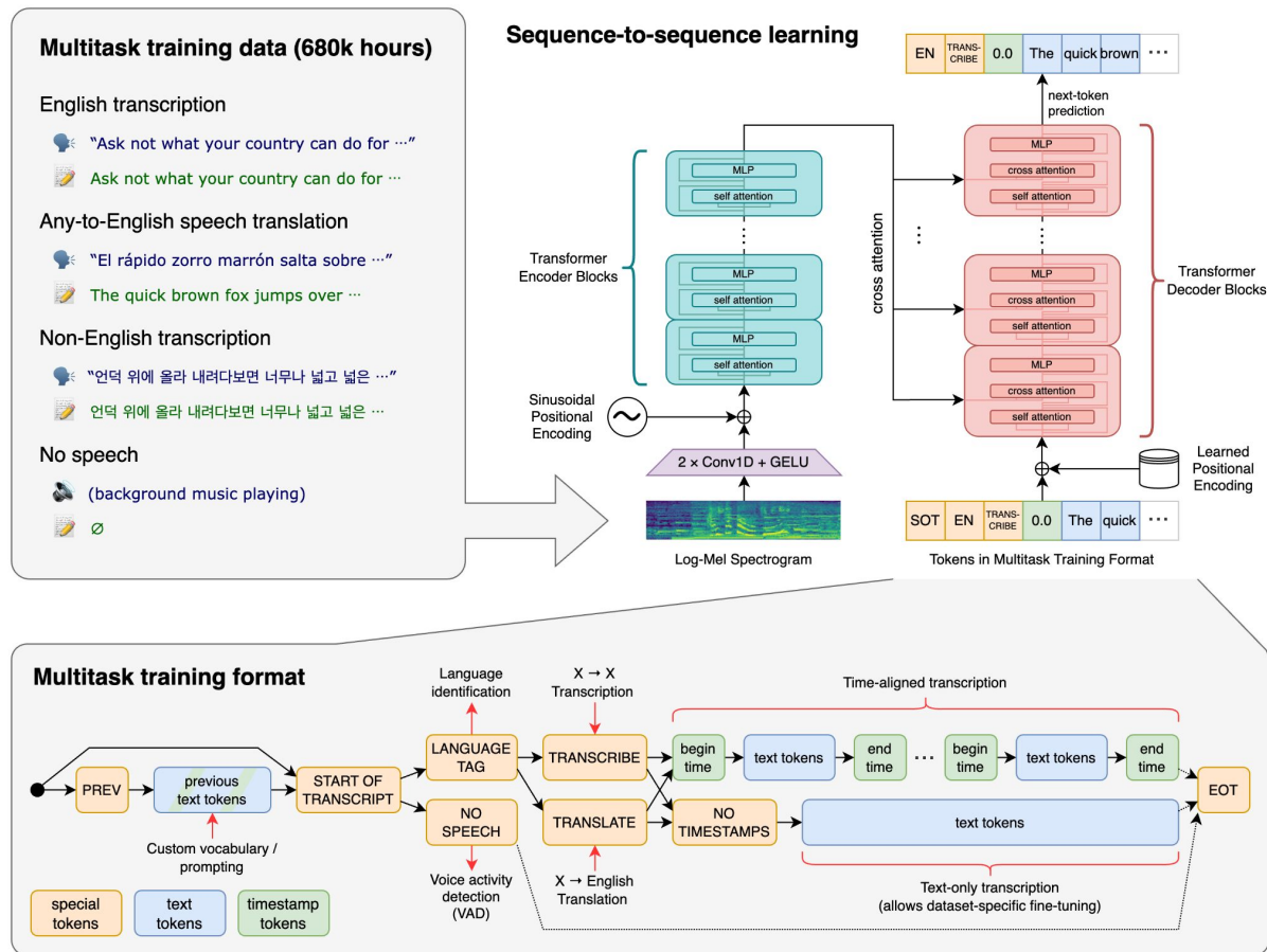
Fig. 2. Whisper Architecture (Alec Radford, 2022)
