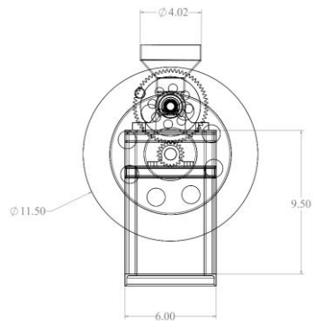
Side View of Oil Expeller
