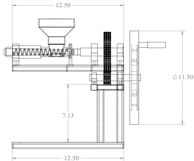
Front View of Oil Expeller
