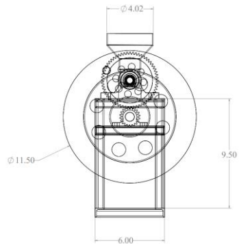
Side View of Oil Expeller
