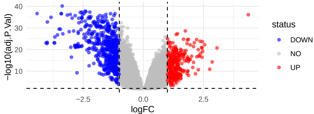
Volcano Plot DEG Kanker Paru
