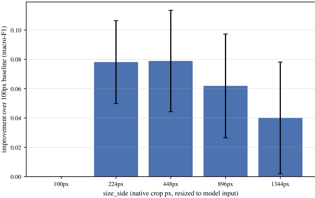
UNI2 colon: macro-F1 improvement over smallest resize
