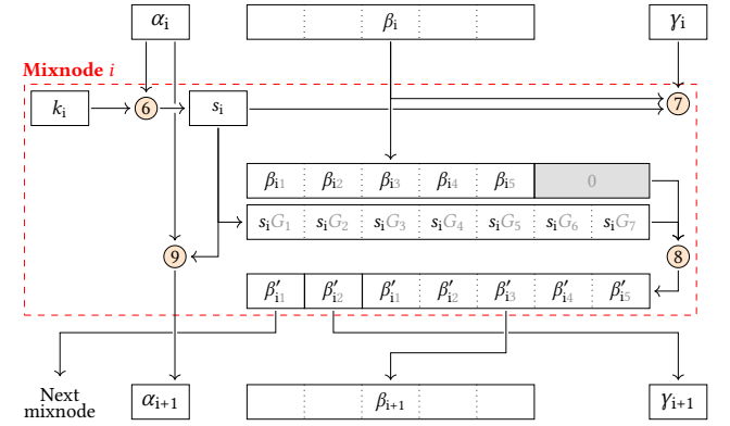
Figure 4: Header processing at mixnode i . Circled numbers \otimes refers to Equation x in the paper.
