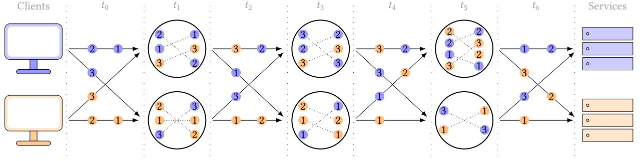
Figure 1: Step-by-step tracing of two clients communicating with services through a 3-layer mixnet. In order to follow paths across each time step, packets are labeled with color and number, respectively indicating the client and message order.
