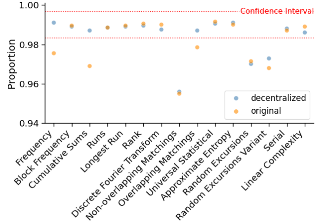
Figure 5: Proportion of successful sequences from our implementation and the original Sphinx implementation over the fifteen NIST SP 800-22 statistical tests (significance level = 0.01).
