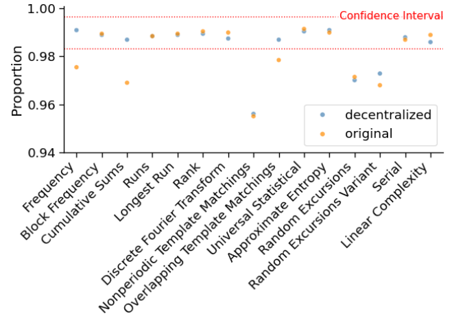
Figure 4: Proportion of successful sequences from our implementation and the original Sphinx implementation over the fifteen NIST SP 800-22 statistical tests (significance level = 0.01).
