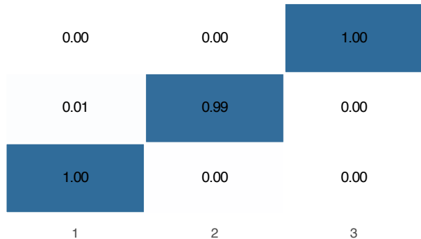
Gaussian HMM, K=3
