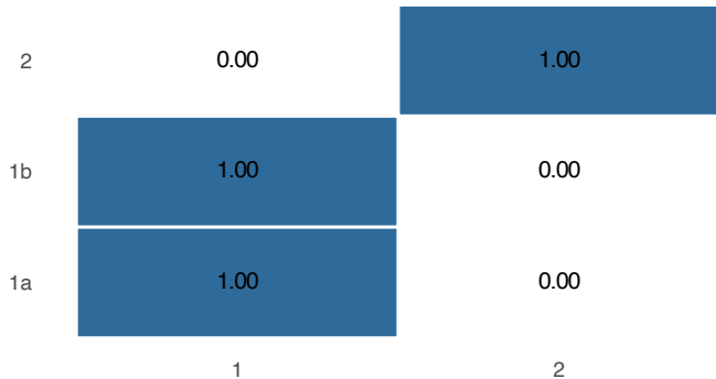
Gaussian HMM, K=2
