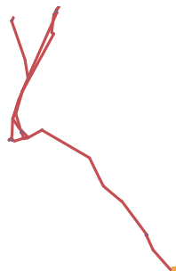
elk-363 Gaussian K=3
