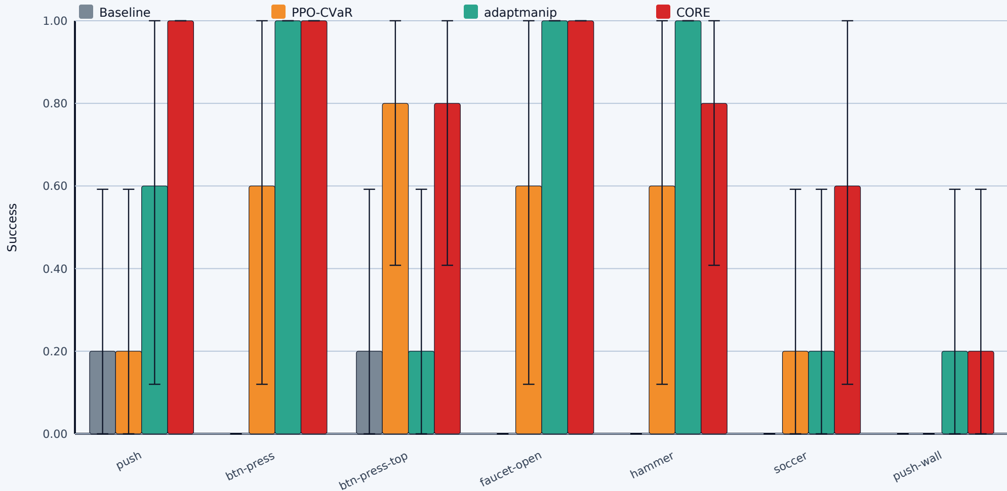
MetaWorld Shifted Task-wise Success
