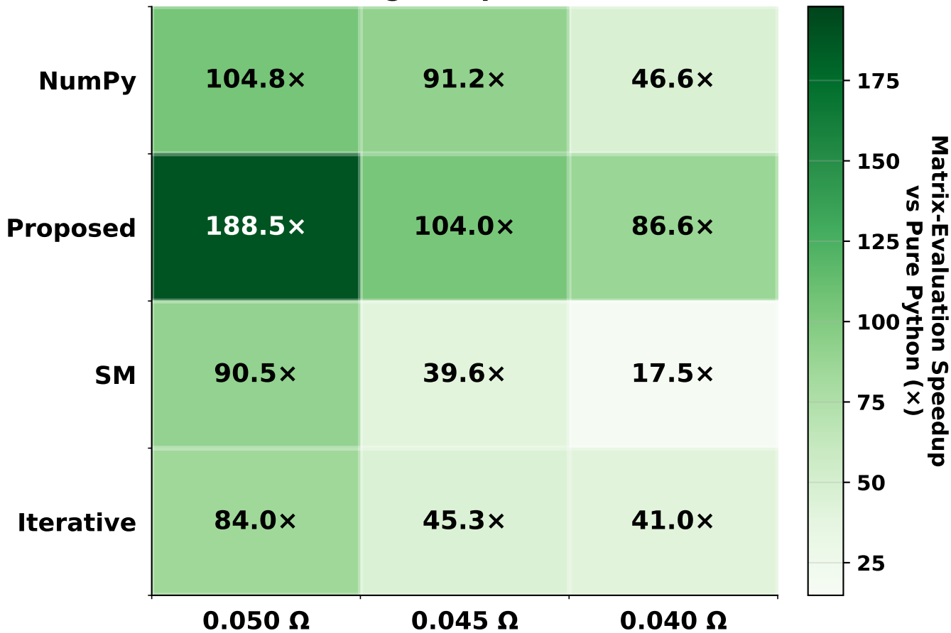
Matrix-Evaluation Speedup Heatmap (Method vs. Target Impedance Threshold)
