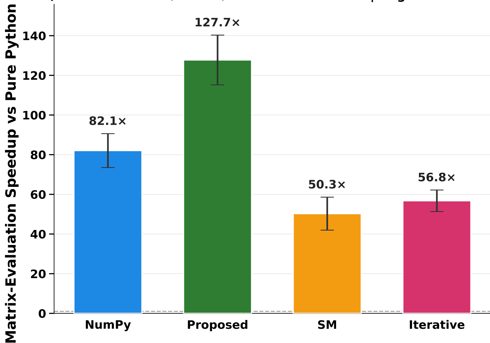
Average Matrix-Evaluation Speedup vs Pure Python (Mean over 0.050 / 0.045 / 0.040 \Omega Thresholds | Higher is Better)
