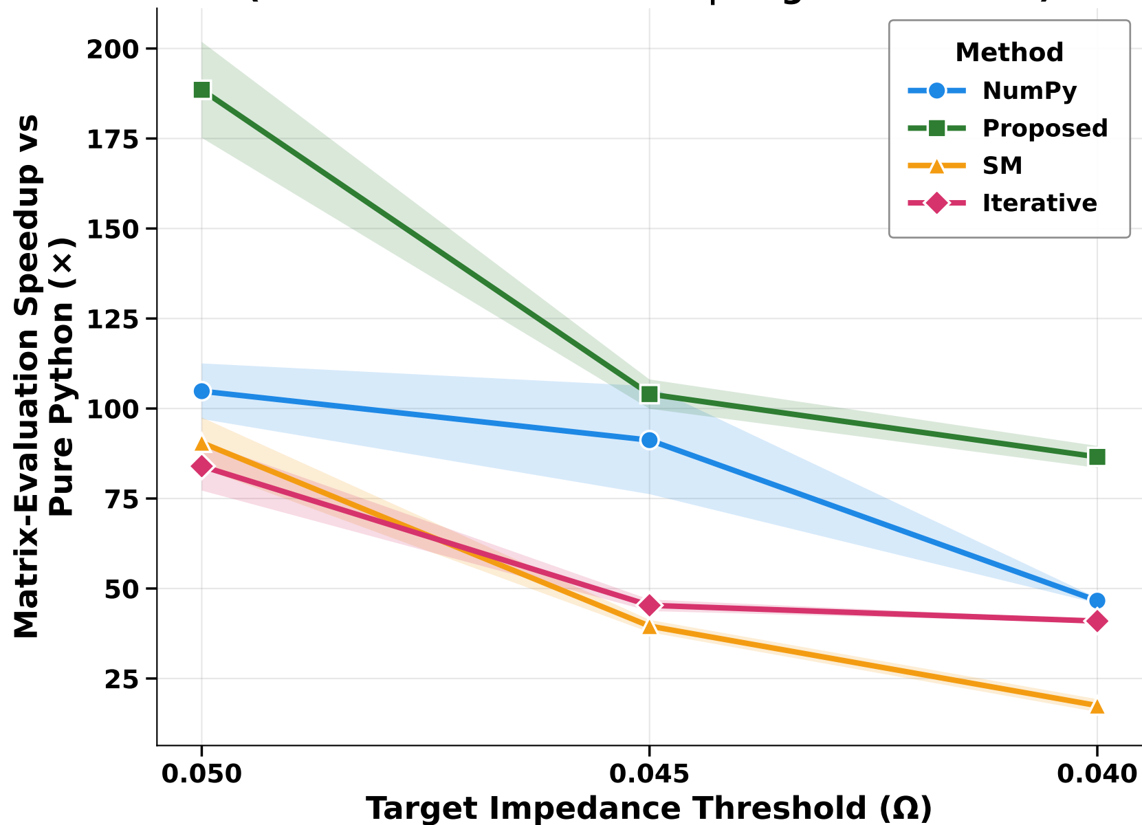
Matrix-Evaluation Speedup vs. Target Impedance Threshold (Shaded Band = 95% CI | Higher is Better)
