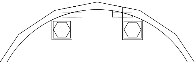
77.076 overall / drawing scale1.100 Vertical24.000; CAD axes YZ
