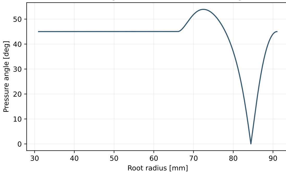
Oscillating follower; numerical screening
