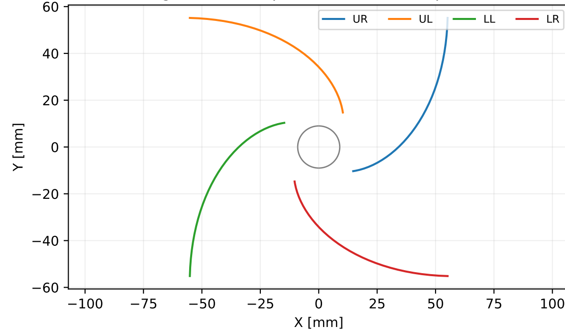
Rigid scroll comparison / no box adaptation
