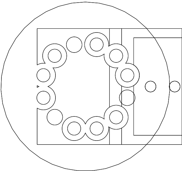
74.972 overall / drawing scale 1.100 Vertical 69.887; CAD axes XZ
