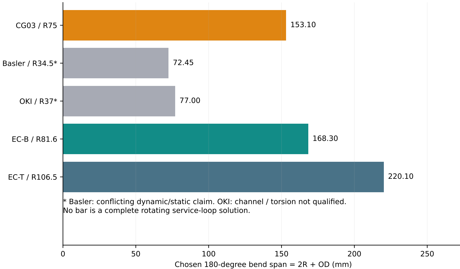
D. Side-cavity scale before wall, clearance, leads or clamps
