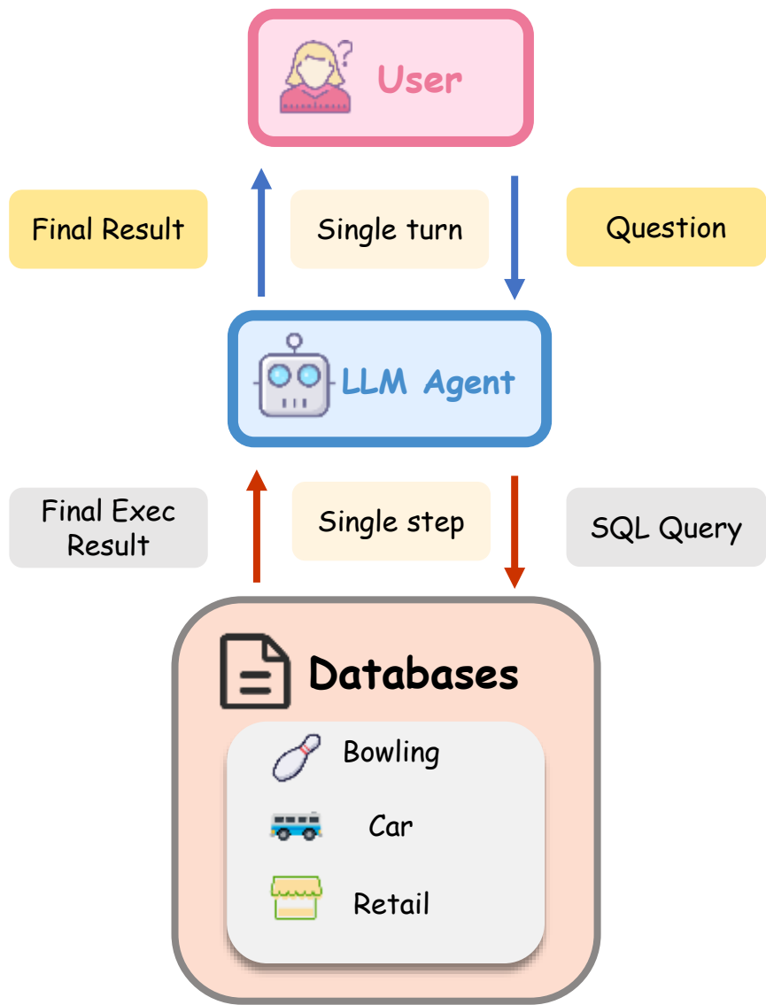
(a) Text-to-SQL
