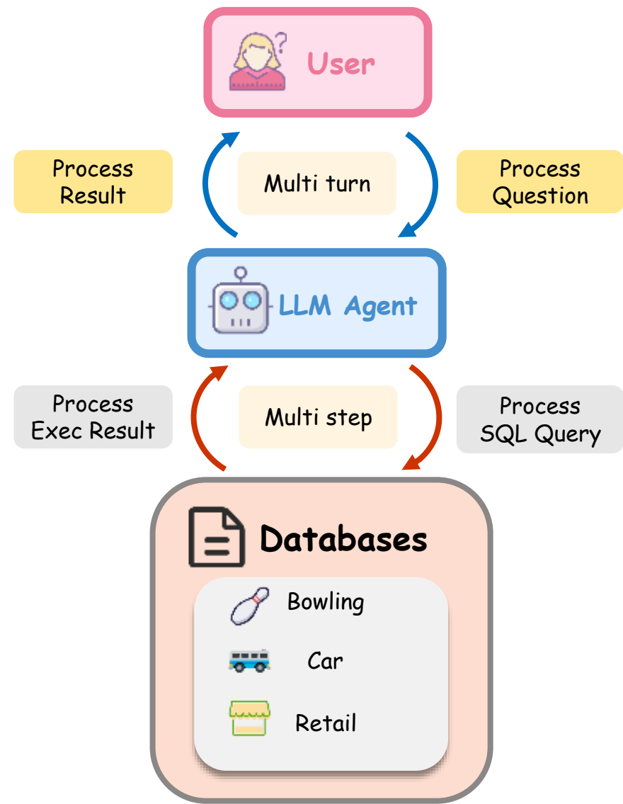
(c) Ours
