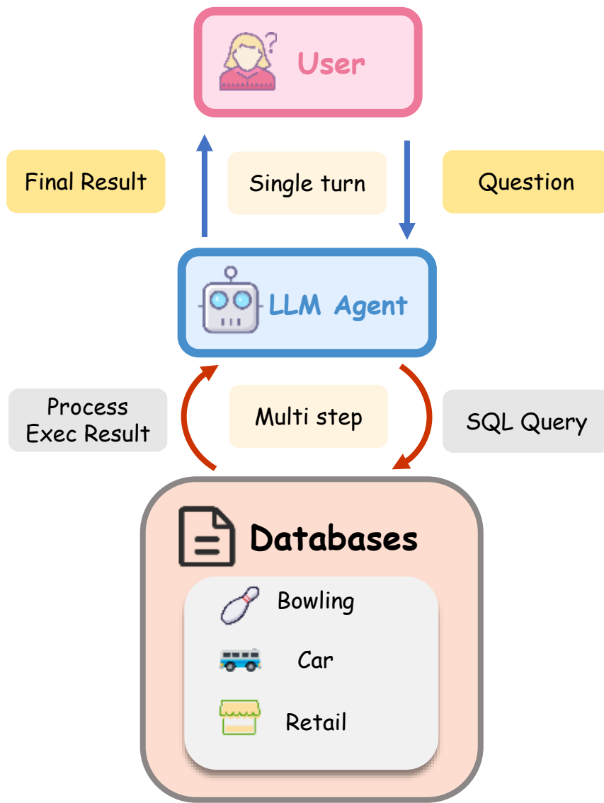
(b) ReAct
