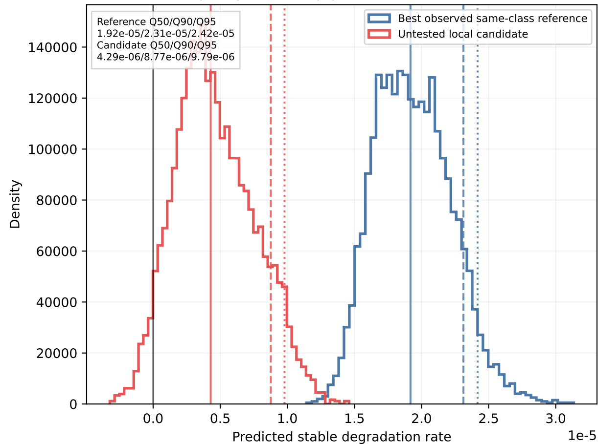
Q2 policy-bootstrap prediction distributions
