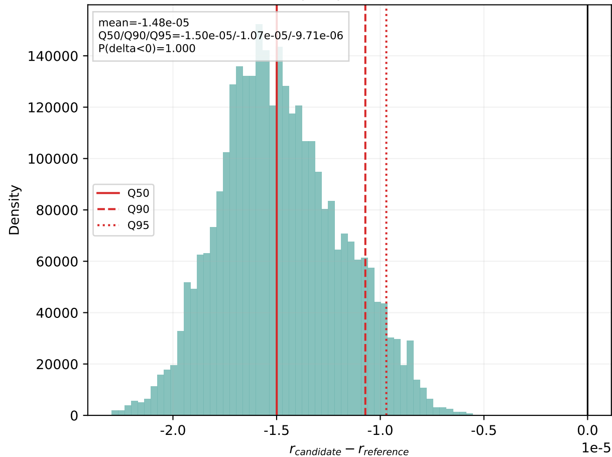
Paired bootstrap improvement distribution
