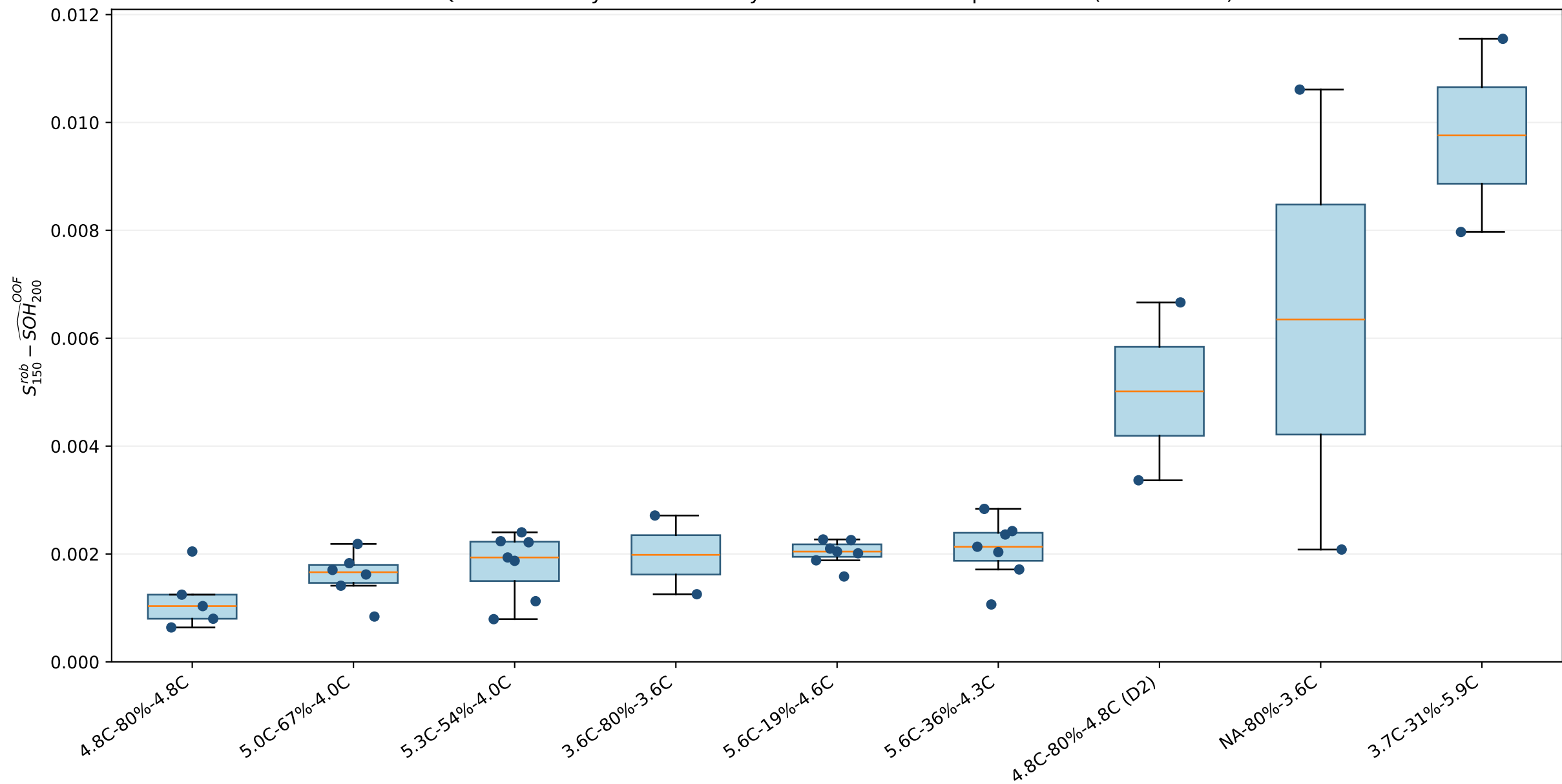
Q3 future-50-cycle consistency: formal outer-LOBO predictions (40 batteries)
