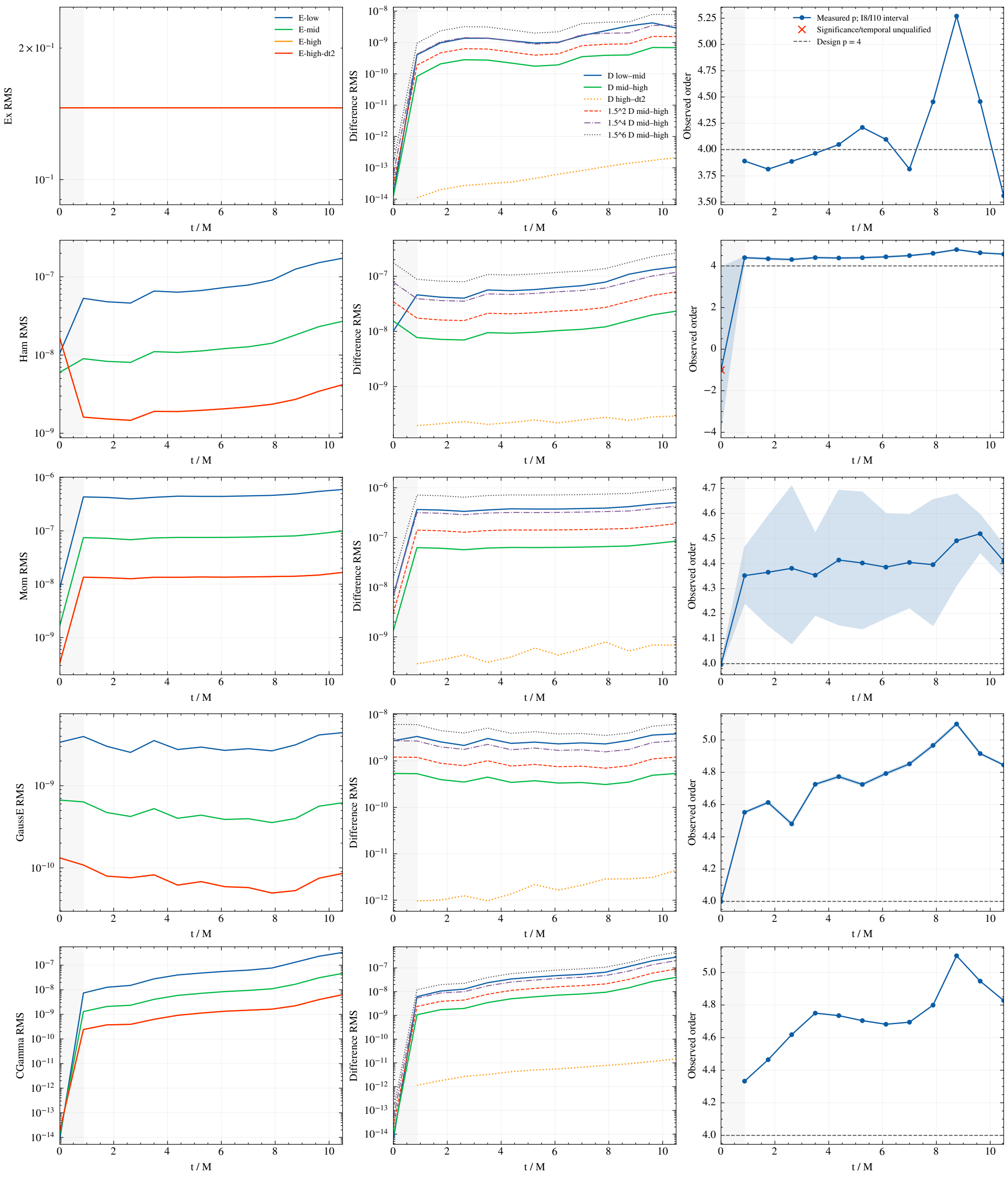
exp-0023: between_rings; coordinate-volume common-support RMS Raw field/constraint norms, pair differences and observed orders; t=0 reported only
