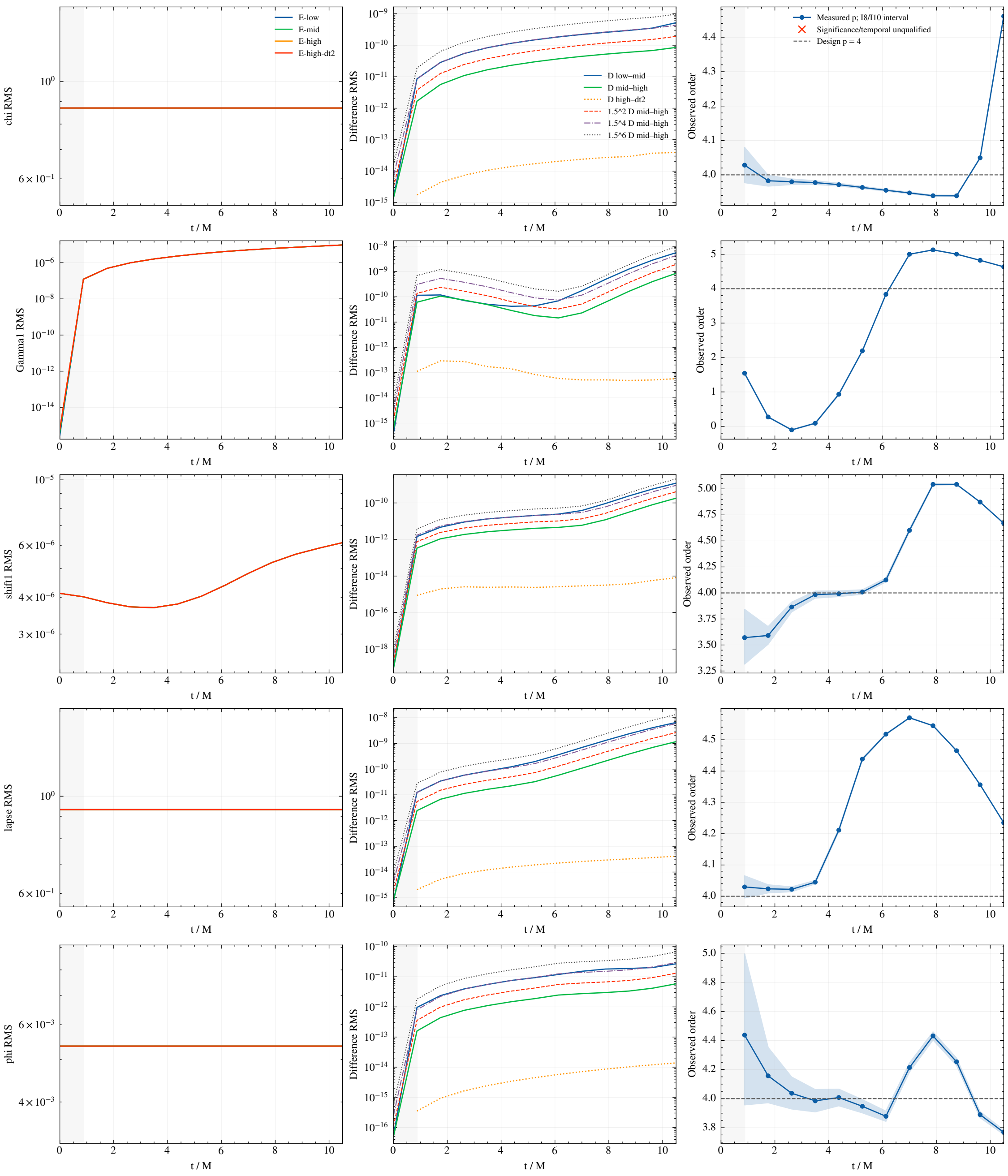
exp-0023: puncture_excluded; coordinate-volume common-support RMS Raw field/constraint norms, pair differences and observed orders; t=0 reported only
