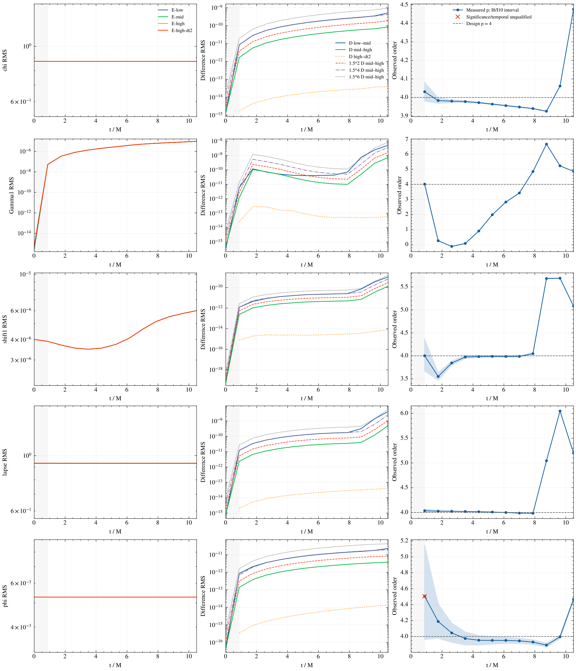
exp-0023: exterior_wake; coordinate-volume common-support RMS Raw field/constraint norms, pair differences and observed orders; t=0 reported only
