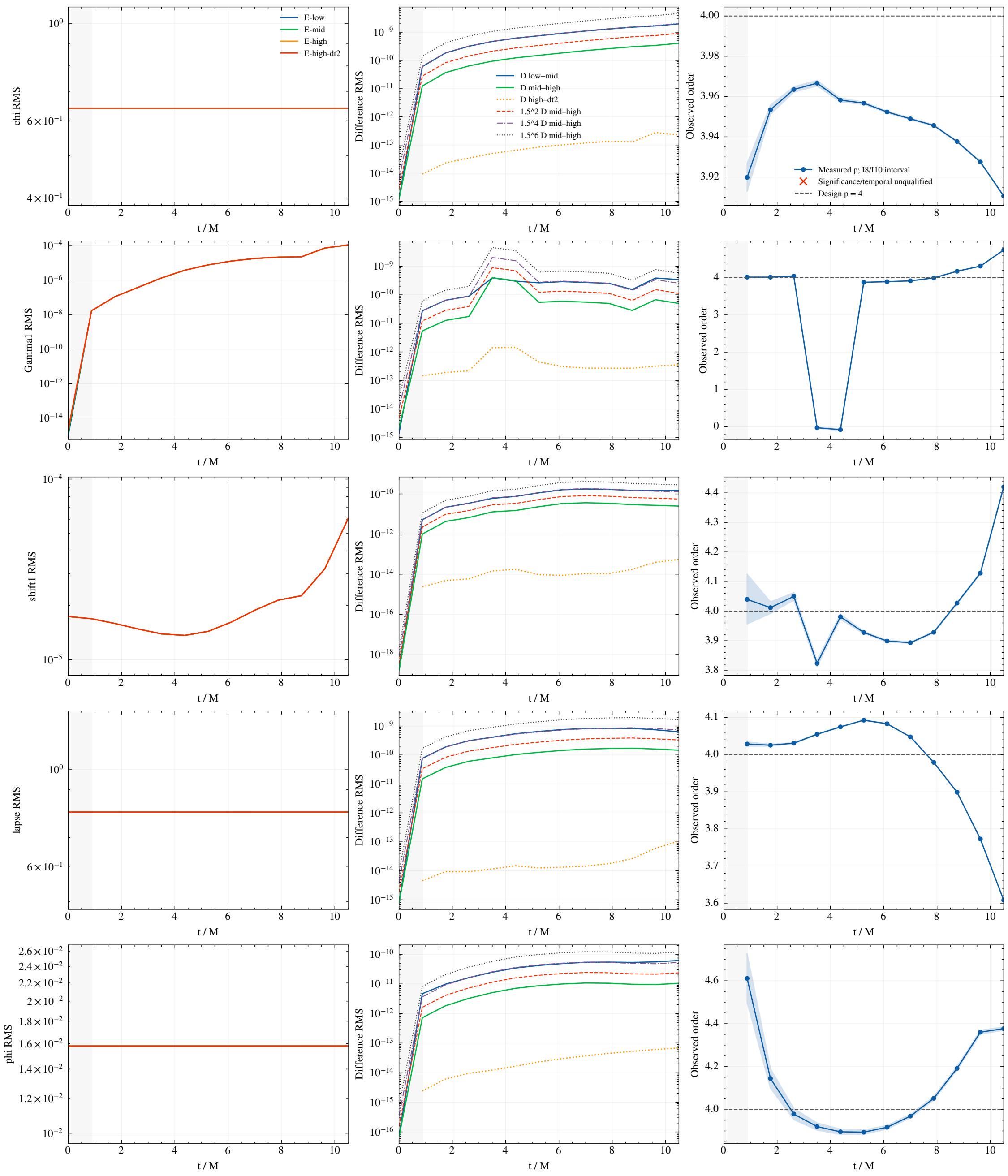
exp-0023: receiving_side_3p5; coordinate-volume common-support RMS Raw field/constraint norms, pair differences and observed orders; t=0 reported only
