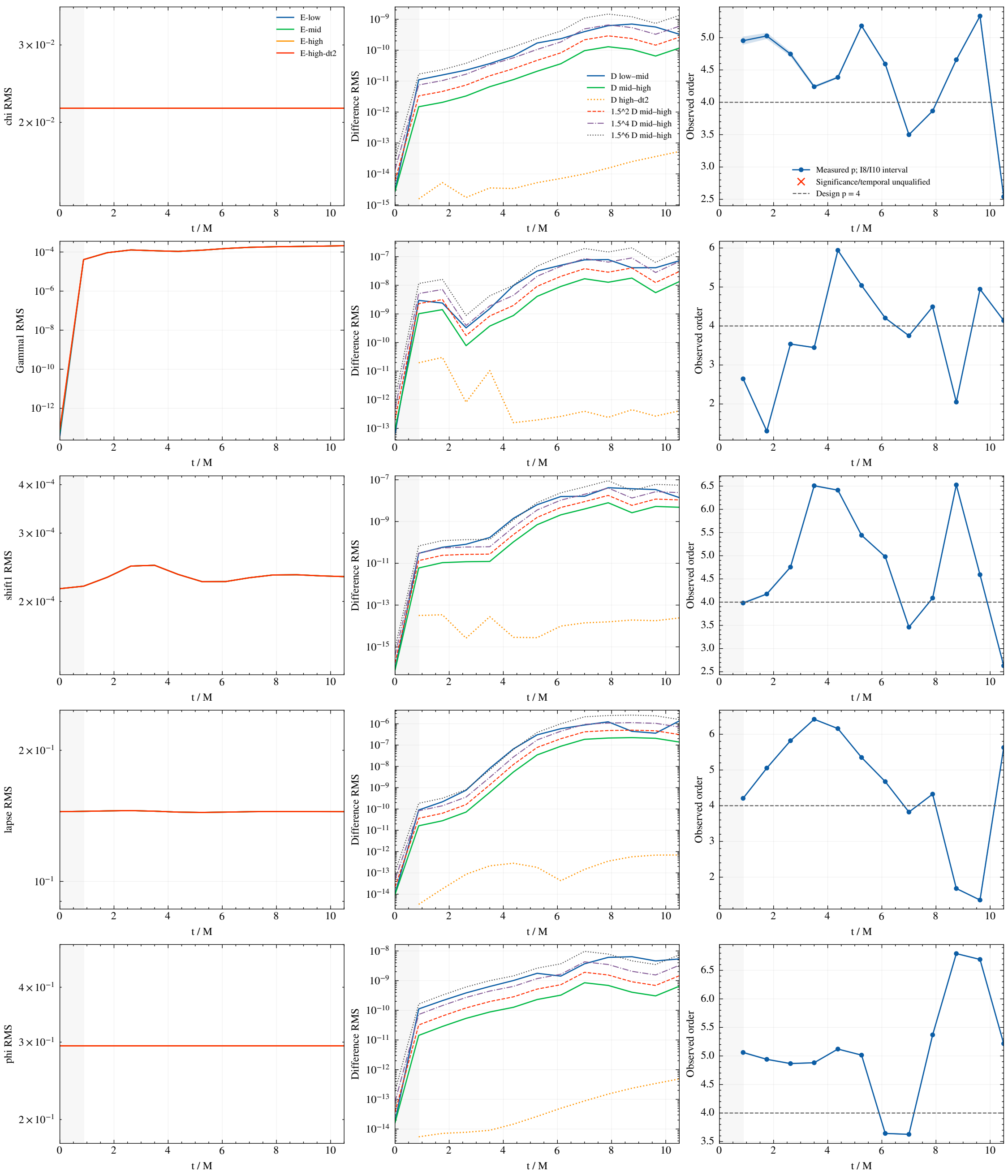
exp-0023: cavity; coordinate-volume common-support RMS Raw field/constraint norms, pair differences and observed orders; t=0 reported only
