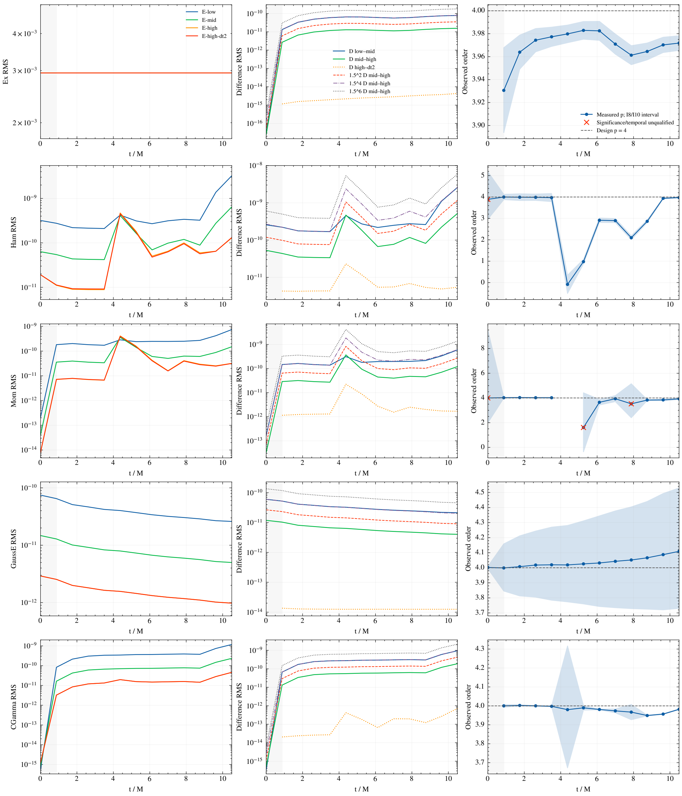
exp-0023: far; coordinate-volume common-support RMS Raw field/constraint norms, pair differences and observed orders; t=0 reported only
