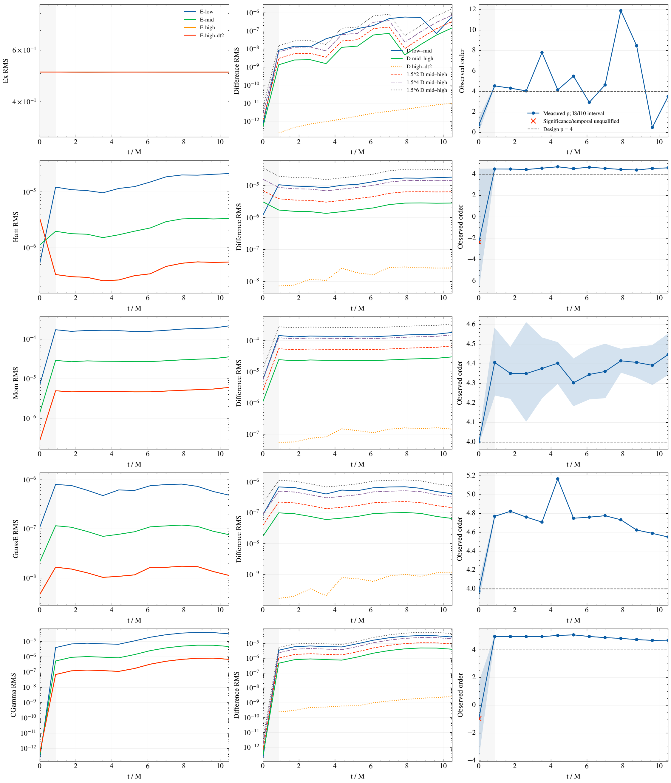
exp-0023: inside_inner_ring; coordinate-volume common-support RMS Raw field/constraint norms, pair differences and observed orders; t=0 reported only
