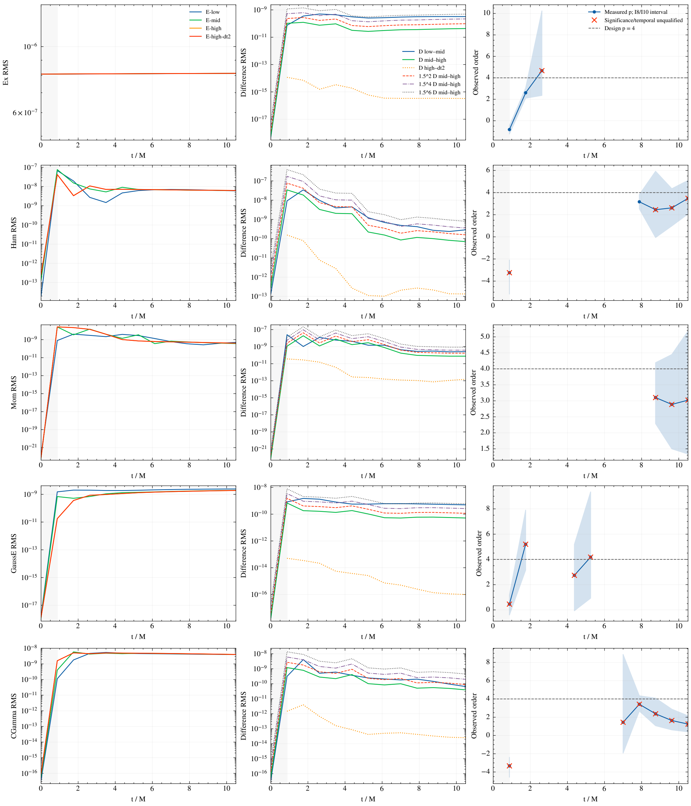
exp-0023: outer_boundary_shell; coordinate-volume common-support RMS Raw field/constraint norms, pair differences and observed orders; t=0 reported only
