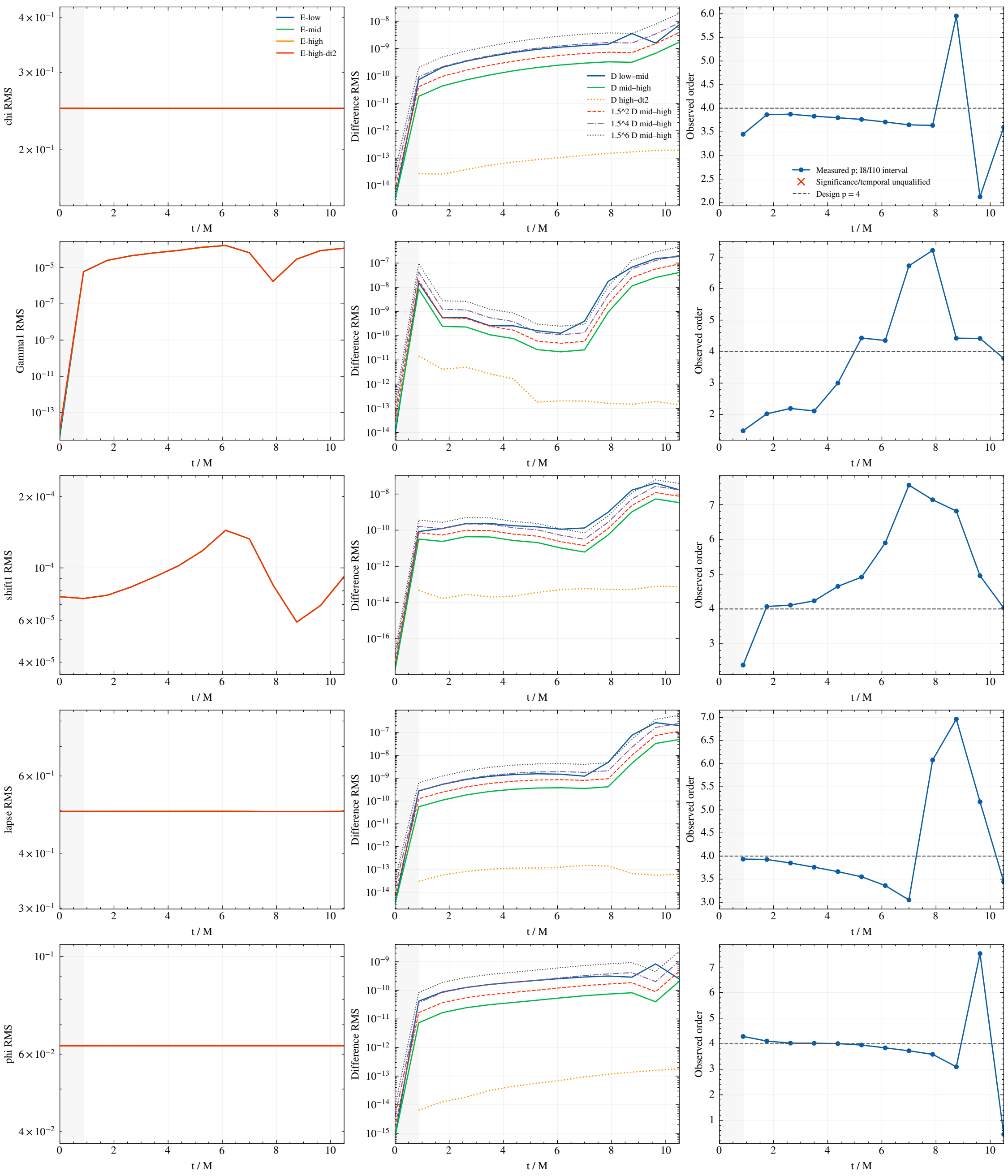
exp-0023: outer_ring_core; coordinate-volume common-support RMS Raw field/constraint norms, pair differences and observed orders; t=0 reported only
