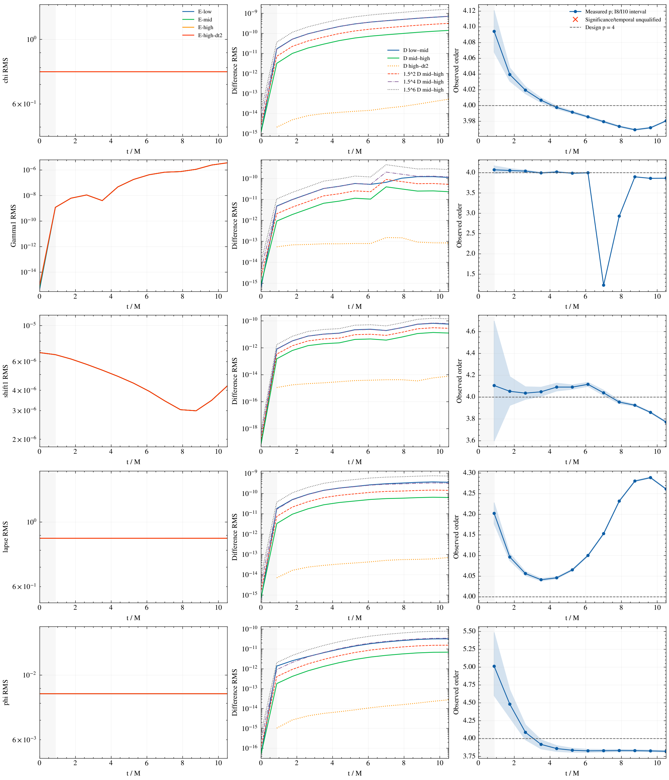
exp-0023: far_core; coordinate-volume common-support RMS Raw field/constraint norms, pair differences and observed orders; t=0 reported only
