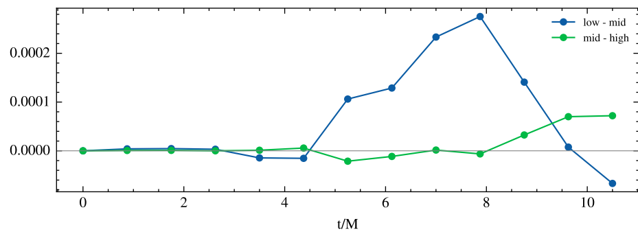
Aww
