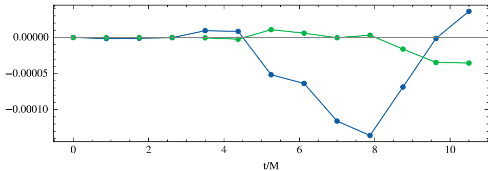
Gamma2
