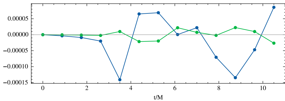
phi
