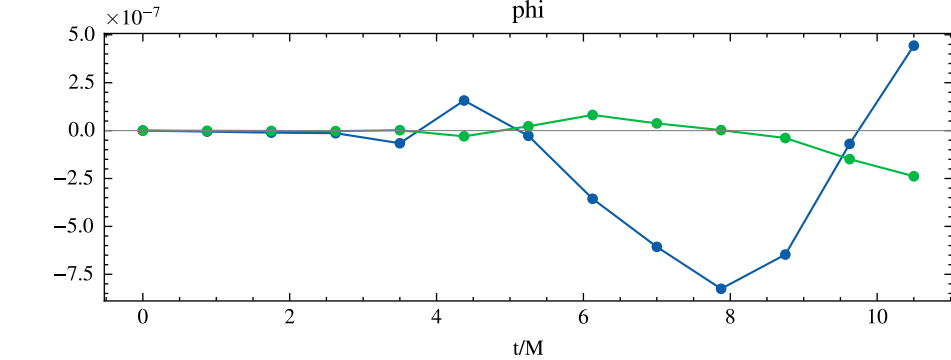
phi
