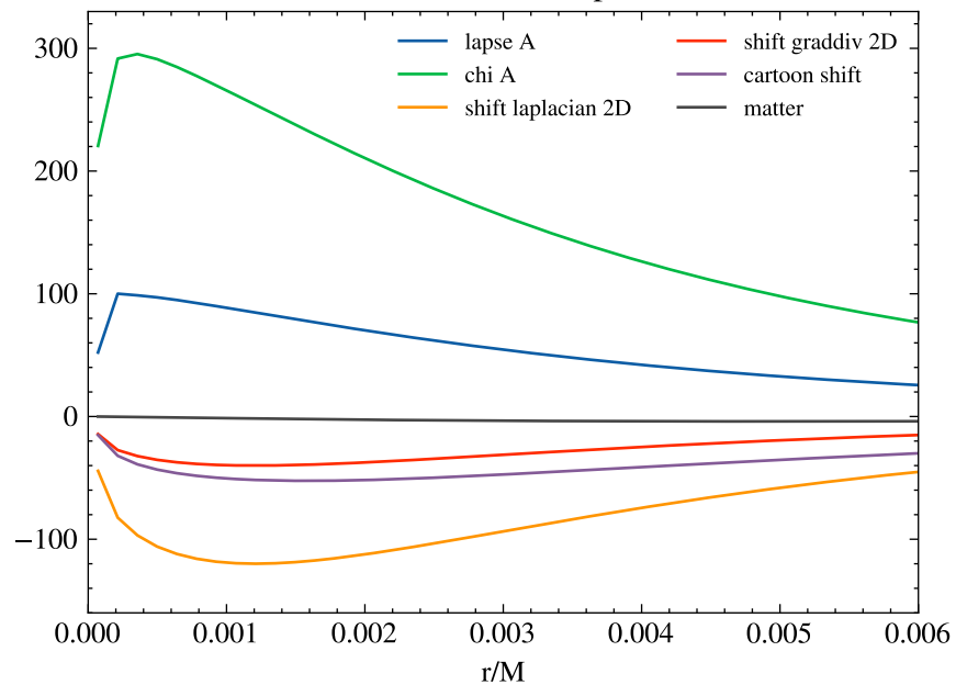
diagonal: L12 term split
