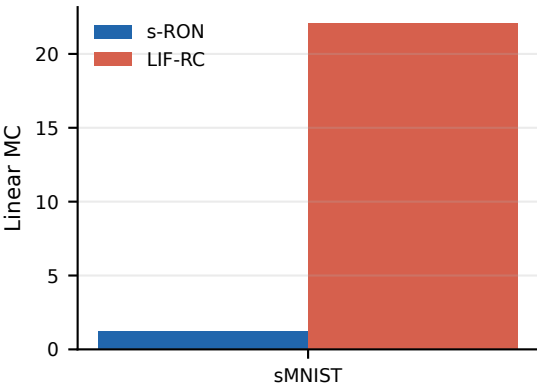
Linear memory capacity
