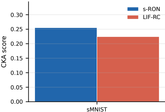
Class-label alignment
