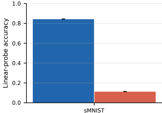
Downstream classifier
