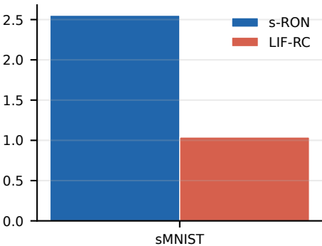
Participation Ratio
