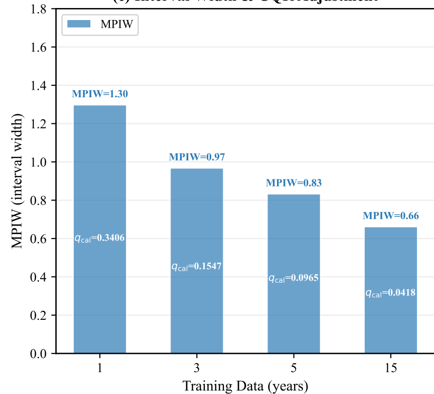
(c) Interval Width & CQR Adjustment
