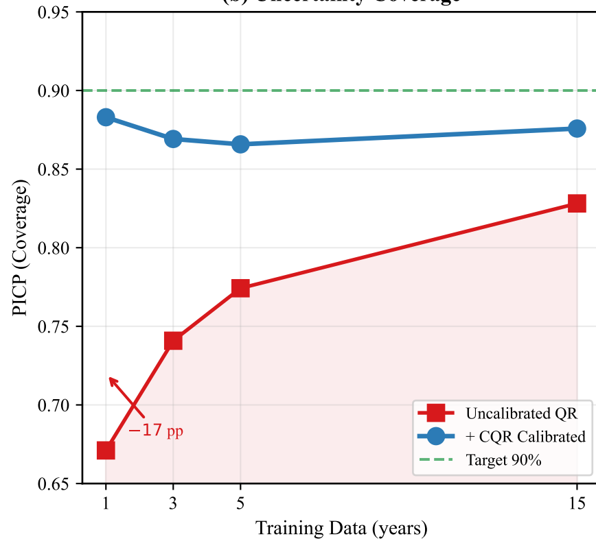
(b) Uncertainty Coverage
