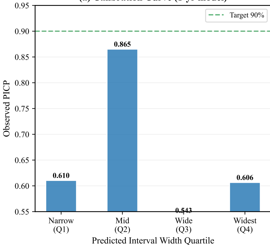
(a) Calibration Curve (1-yr model)
