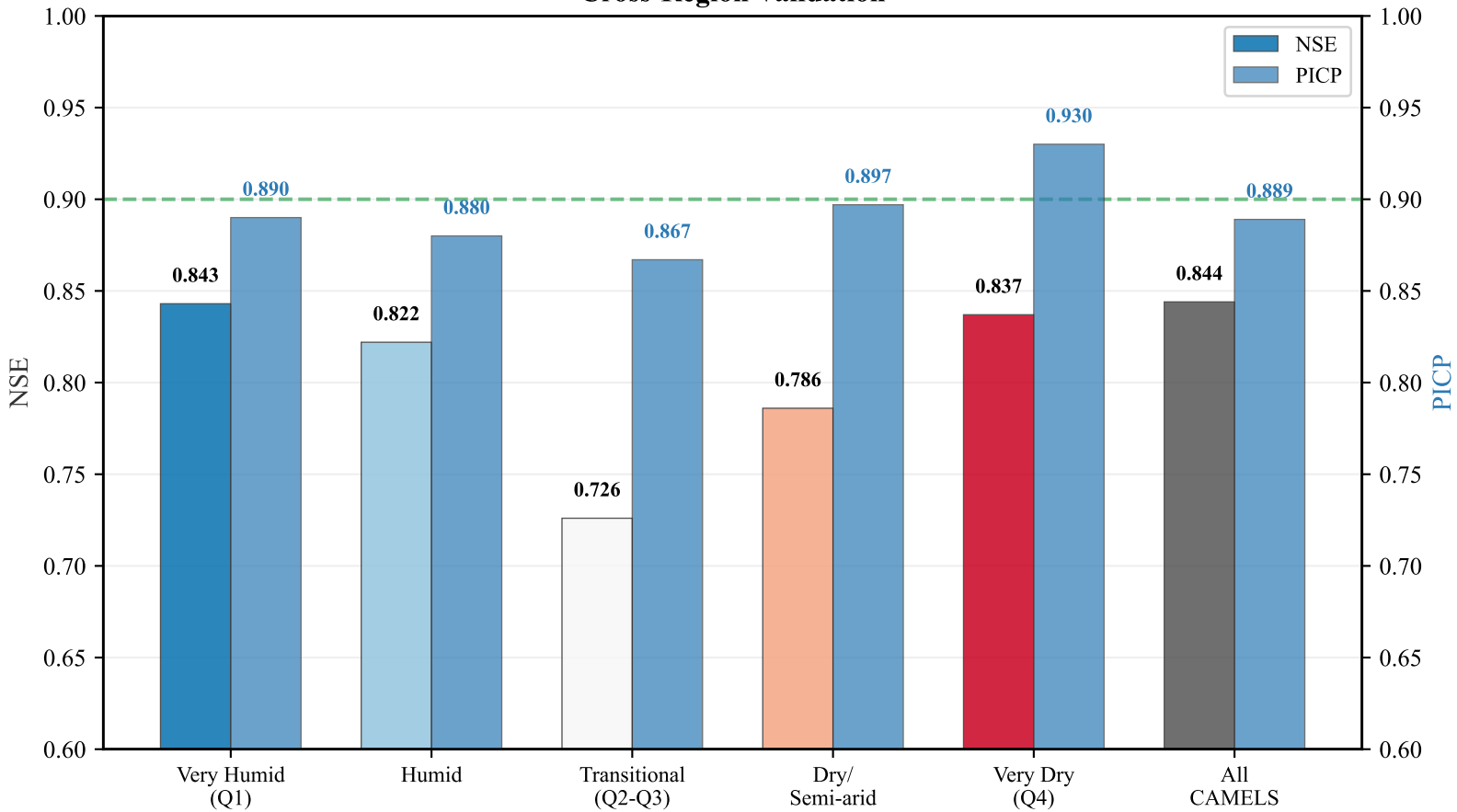
Cross-Region Validation
