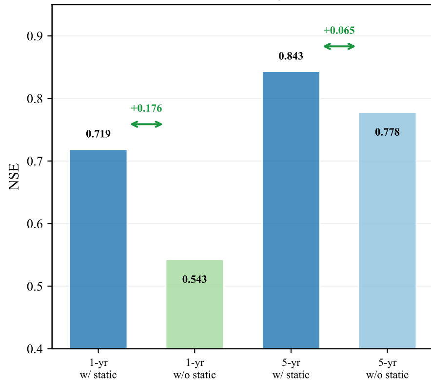
(b) Static Embedding Ablation
