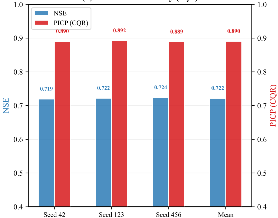
(a) Multi-Seed Stability (1-yr)
