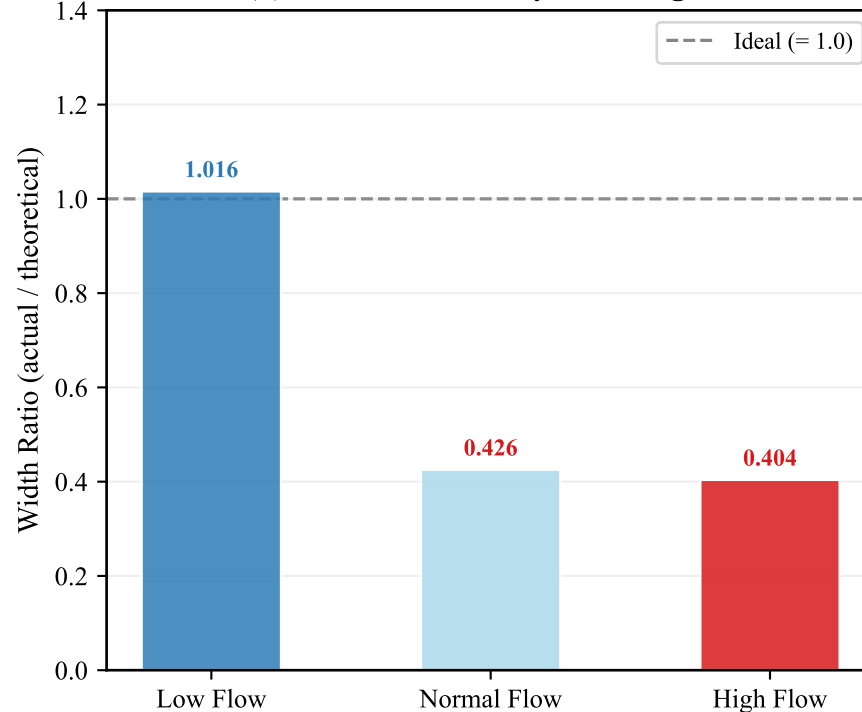
(b) Overconfidence by Flow Regime
