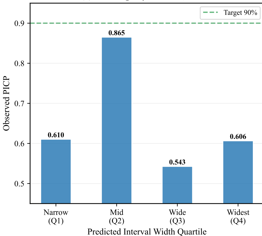
(a) Coverage by Width Quartile
