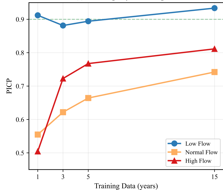
(c) Coverage by Flow Regime
