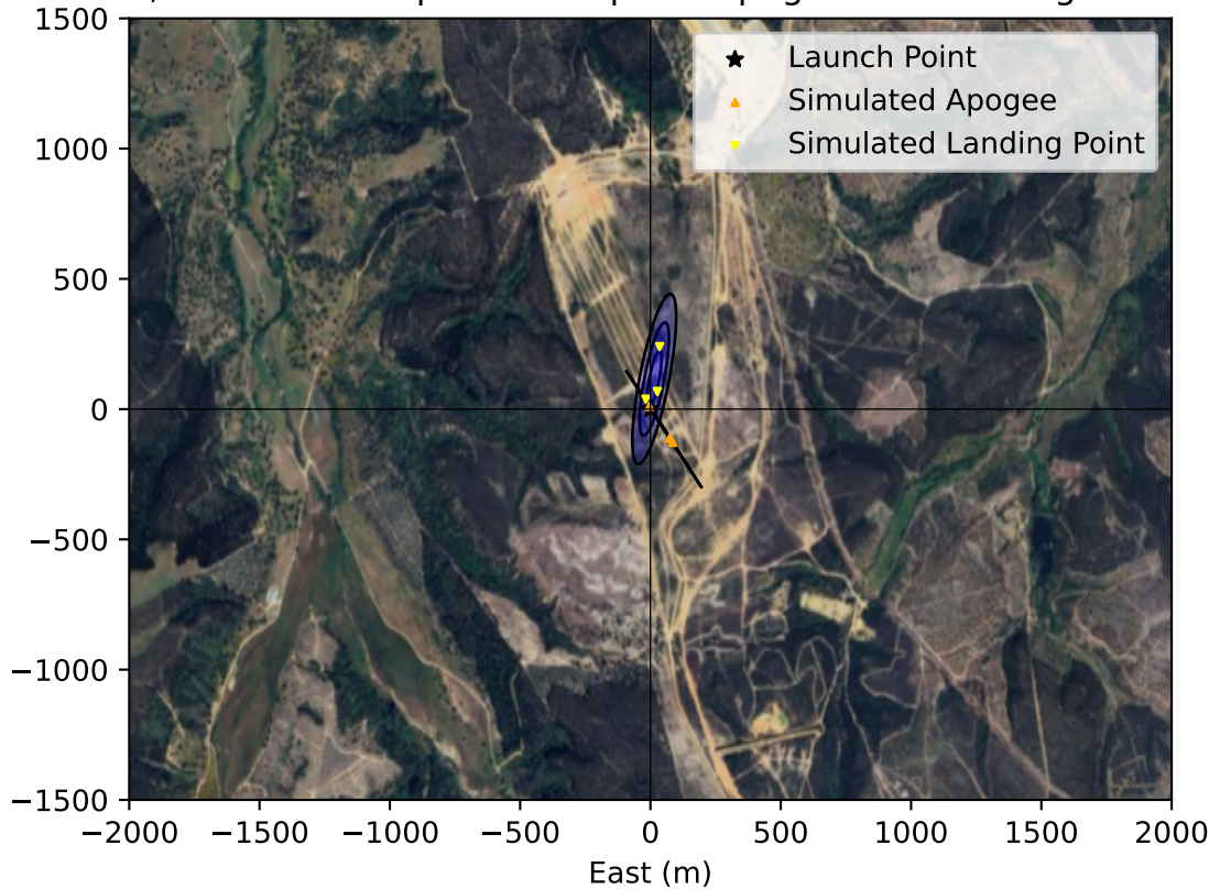
1 \sigma , 2 \sigma and 3 \sigma Dispersion Ellipses: Apogee and Landing Points
