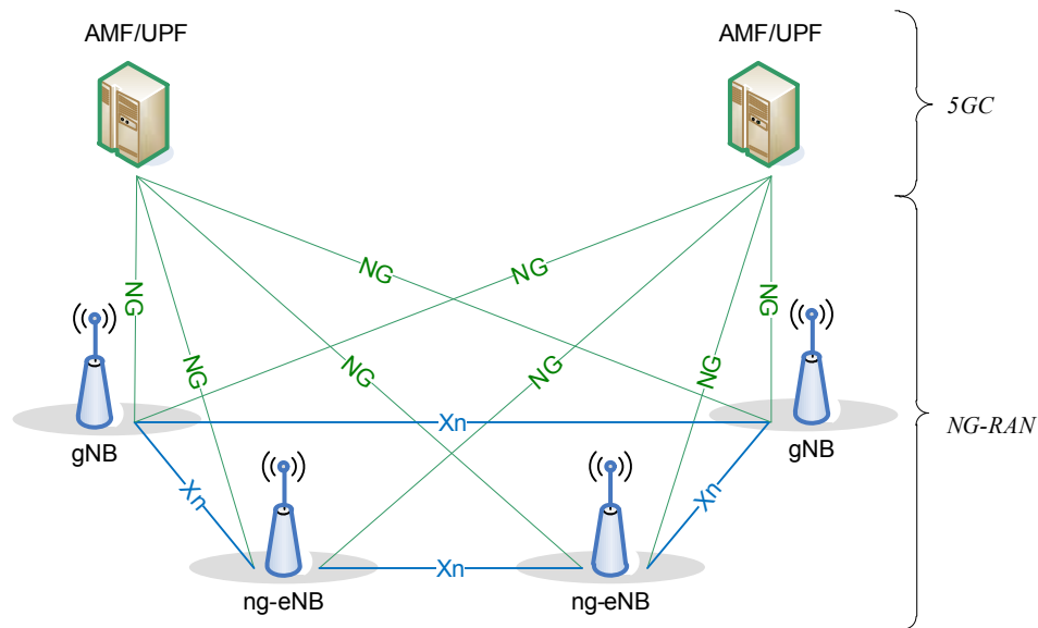
Figure 4.1-1: Overall Architecture
