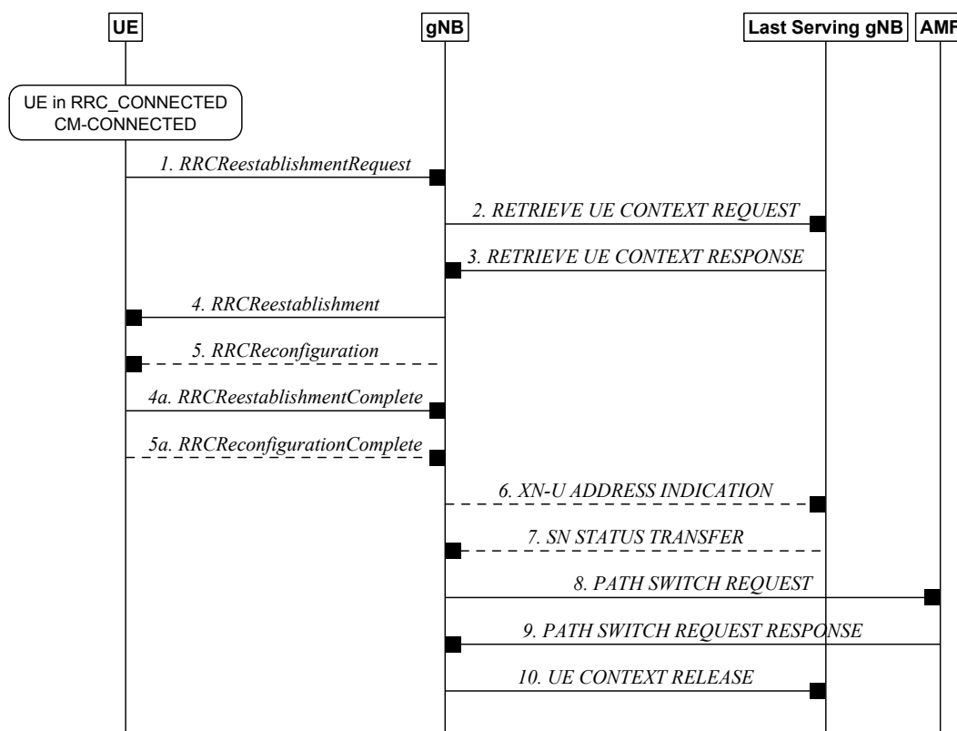
Figure 9.2.3.3-1: Re-establishment procedure
