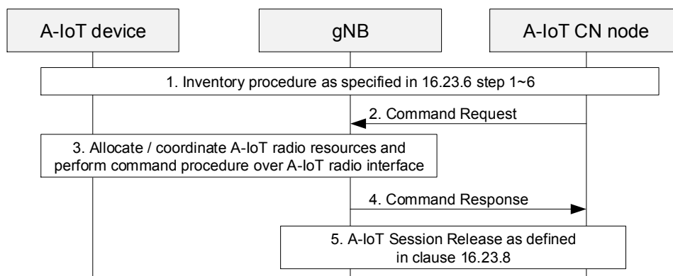
Figure 16.23.7-1: Command procedure
