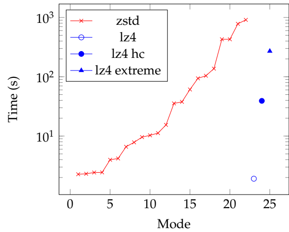
Figure 12: Logarithmic plot of trace compression times for different compression modes (see table 7).
