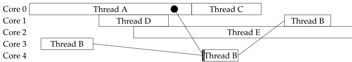
Figure 19: Thread migration and wake up.
