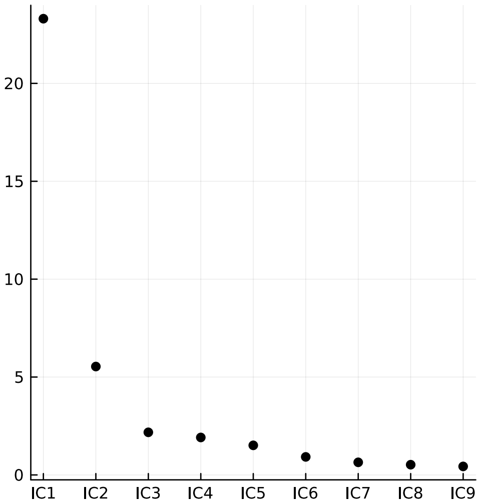
Generalized kurtosis
