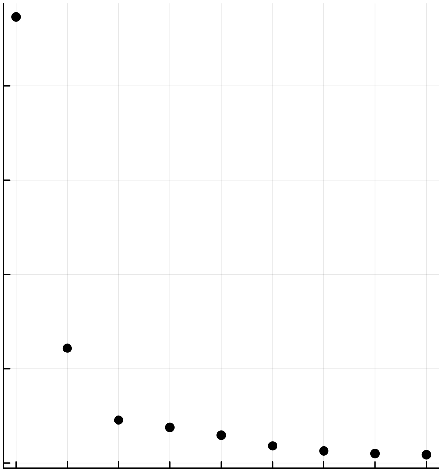
Generalized kurtosis
