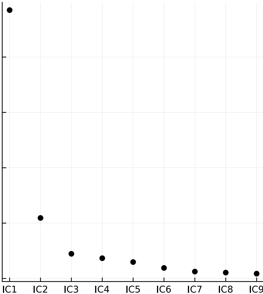
Generalized kurtosis
