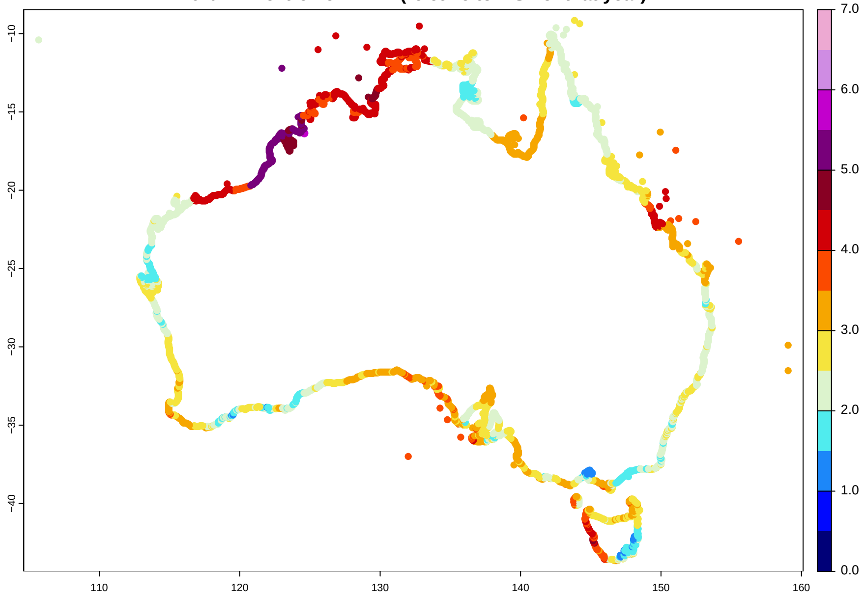
10% AEP extreme MTWL (reletive to MSL of that year)
