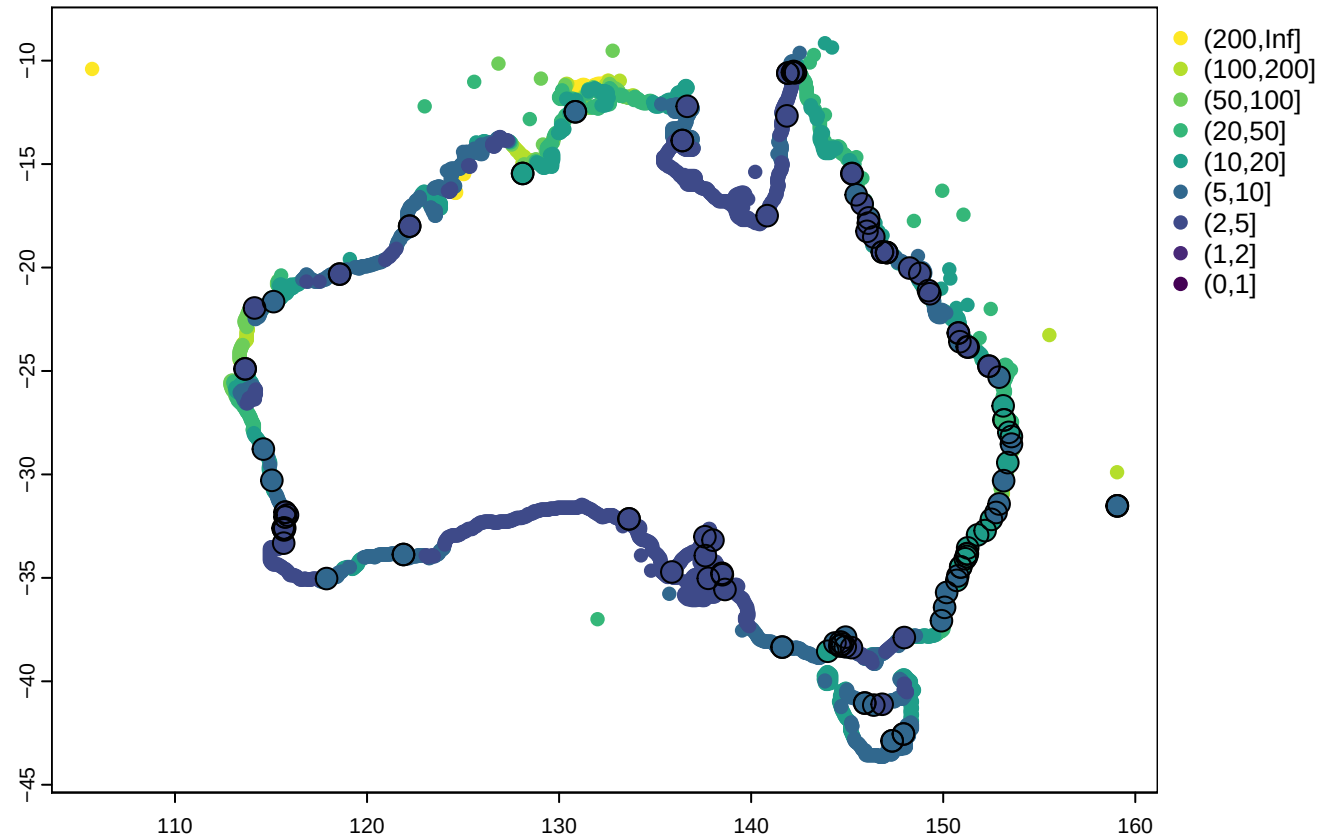
Extreme SWL multiplication factor for 0.14m of SLR
