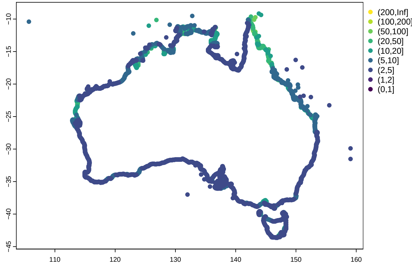
Extreme MTWL multiplication factor for 0.32m of SLR
