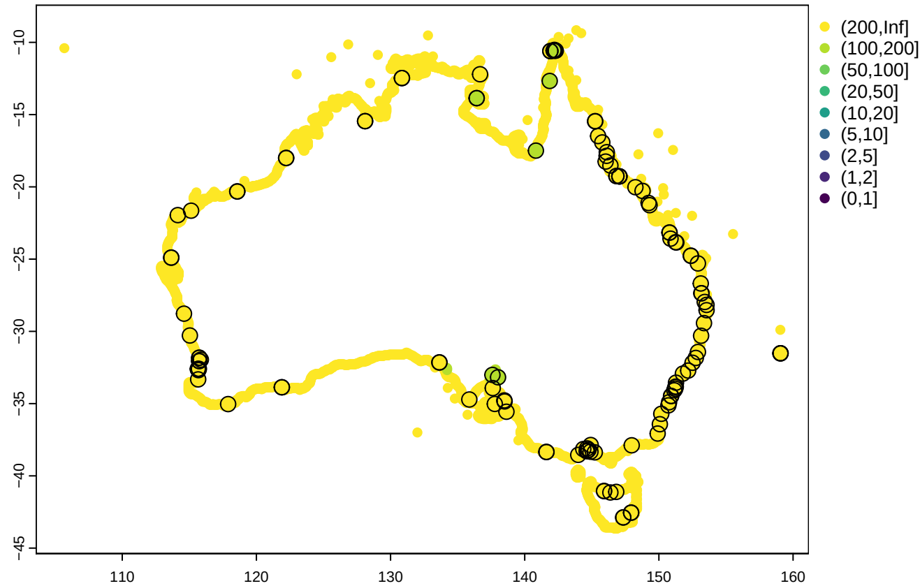
Extreme SWL multiplication factor for 0.9m of SLR
