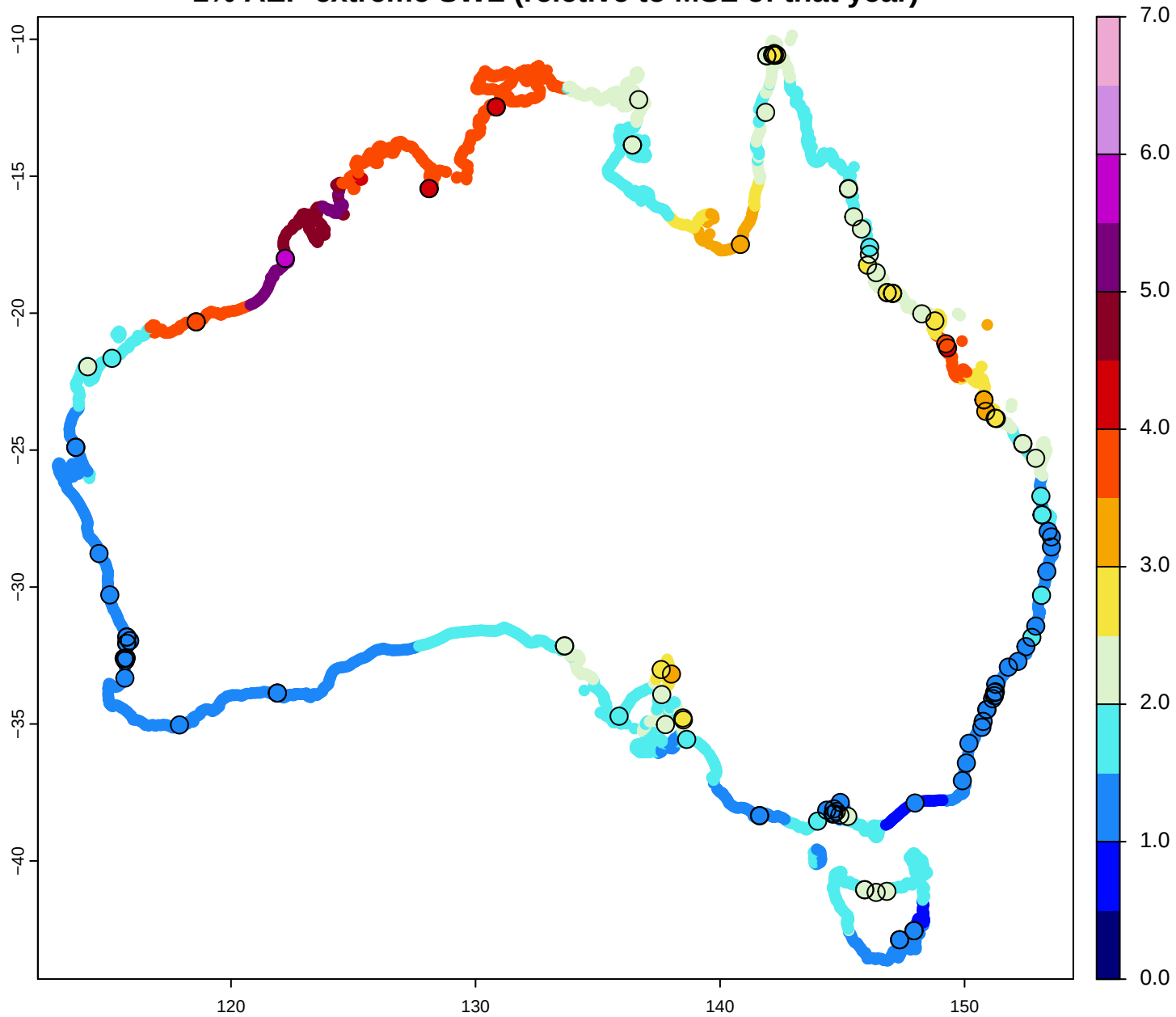
1% AEP extreme SWL (relative to MSL of that year)
