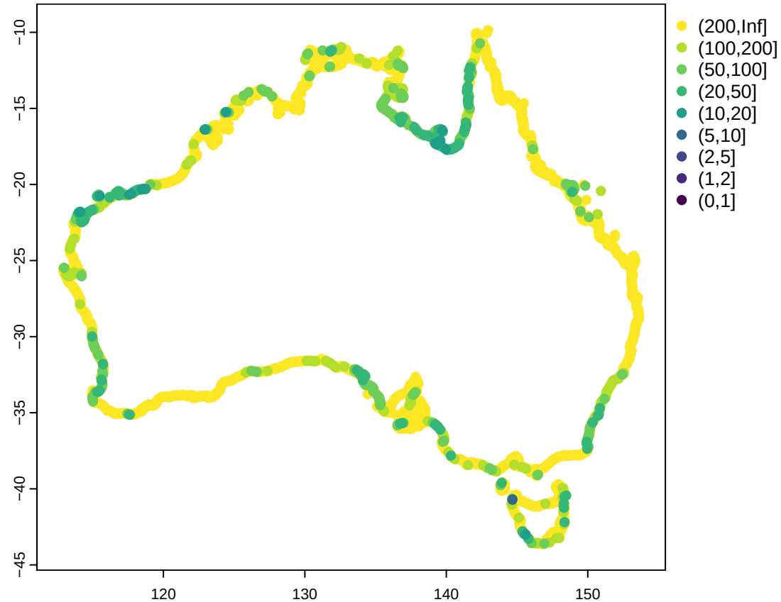
Extreme MTWL multiplication factor for 1m of SLR
