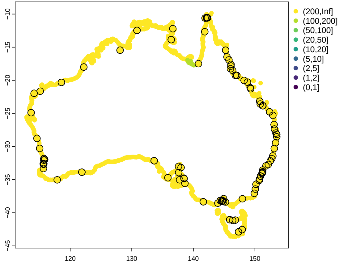
Extreme SWL multiplication factor for 1m of SLR
