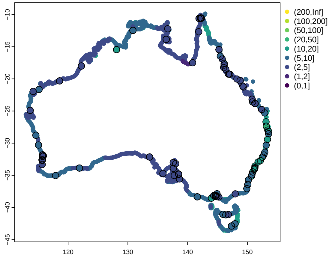
Extreme SWL multiplication factor for 0.14m of SLR
